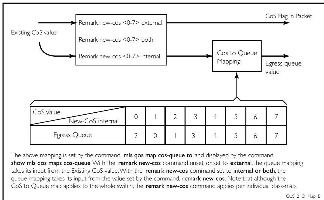
Figure 37-1: Remarking and the CoS to Q map
