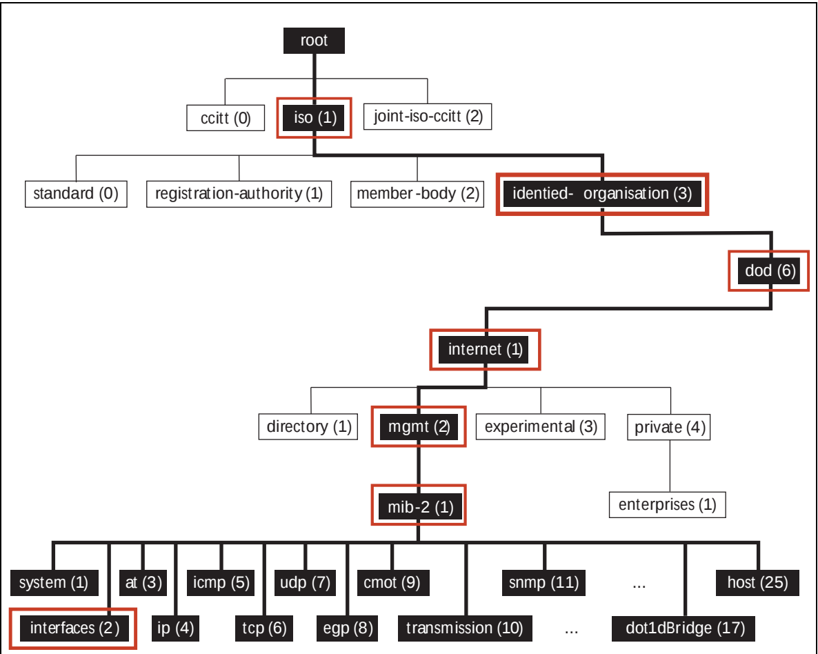
Figure 2: Top levels of the Internet-standard Management Information Base (MIB)
